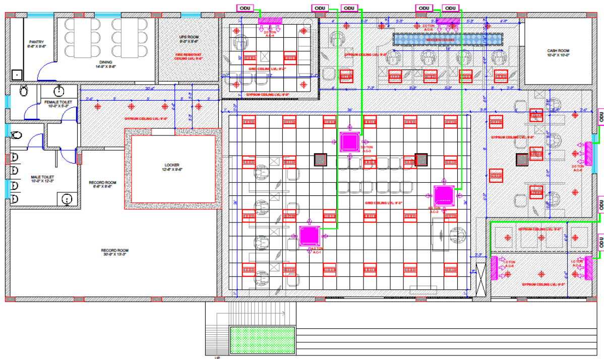
AC LAYOUT
